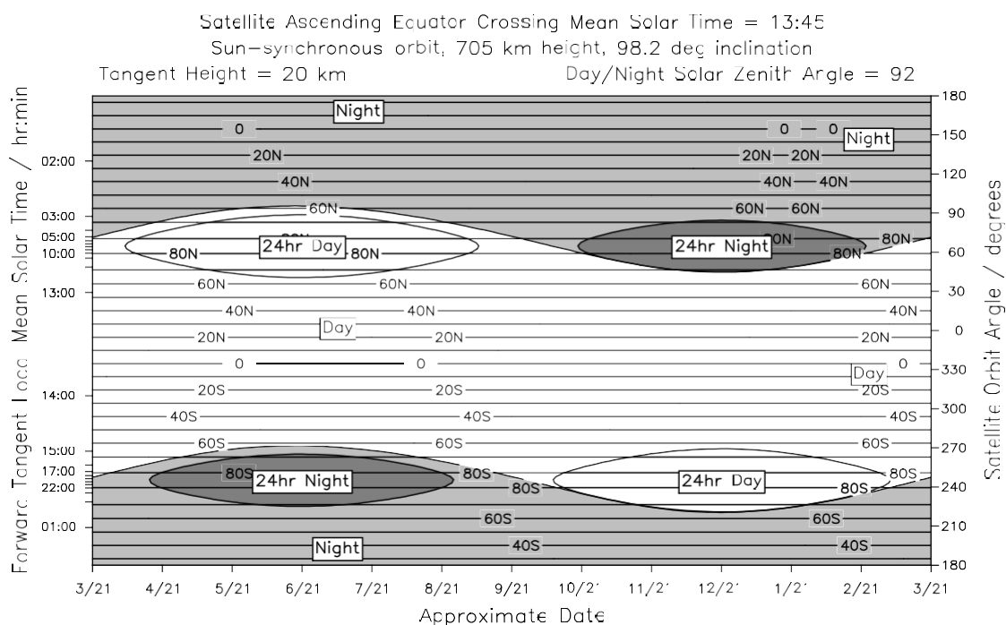
Figure 6-5. Variation, over an annual cycle, of the latitude range where MLS measurements are in day and in night. The horizontal axis gives the approximate date. The right hand vertical axis gives the orbit angle (defined as zero when the satellite is over the equator); the left hand vertical axis gives the corresponding local mean solar time at the (forward) tangent point of MLS observations. Horizontal lines give the latitude of the MLS tangent point, and the day-night boundary is defined as 92^\circ local solar zenith angle.
